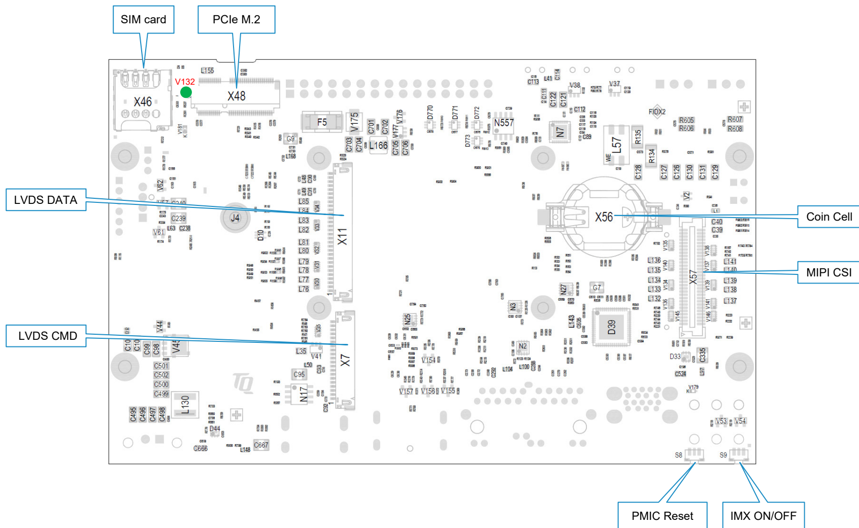
Figure 3: MBa8MPxL interfaces bottom
