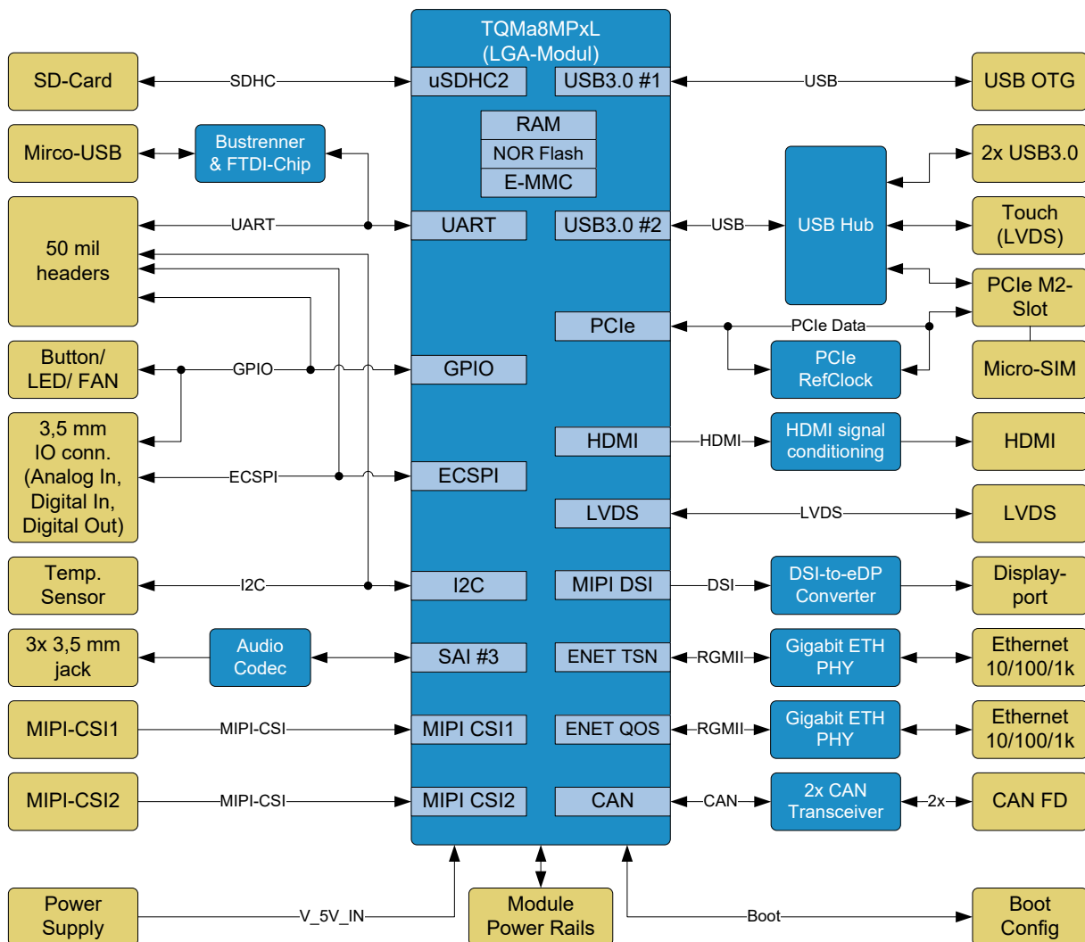
Figure 1: Block diagram MBa8MPxL
