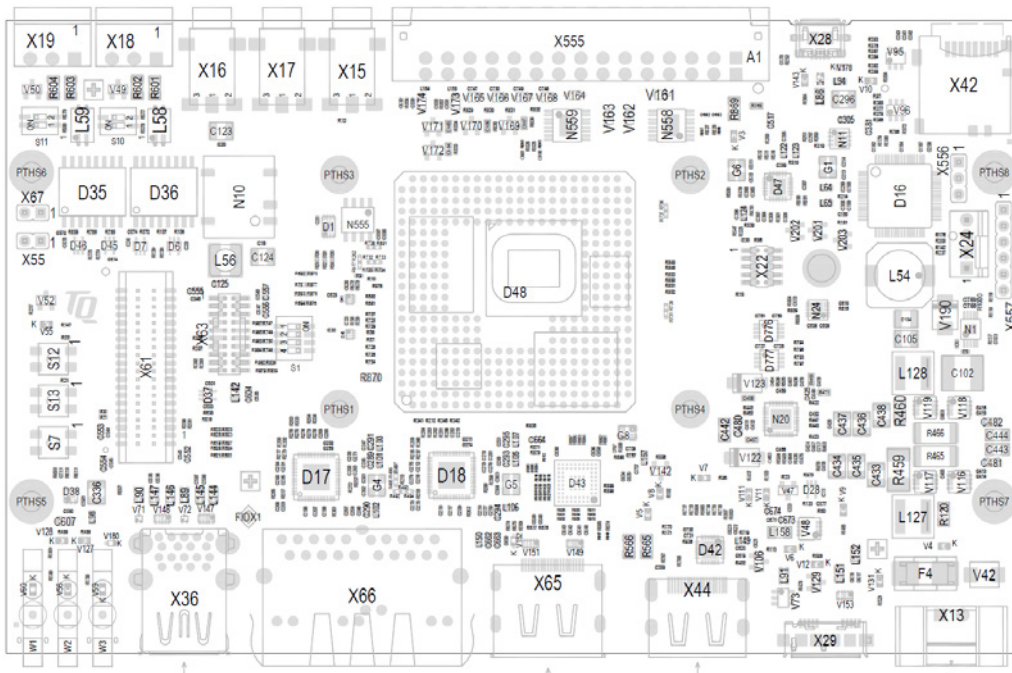
Figure 25: MBa8MPxL component placement top
