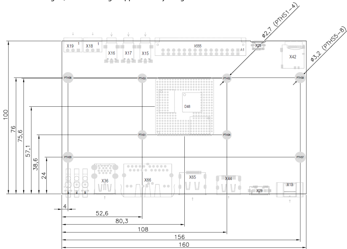
Figure 24: MBa8MPxL dimensions
