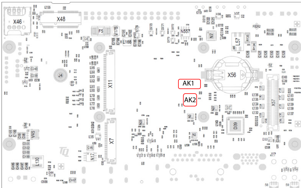
Figure 26: MBa8MPxL component placement bot
