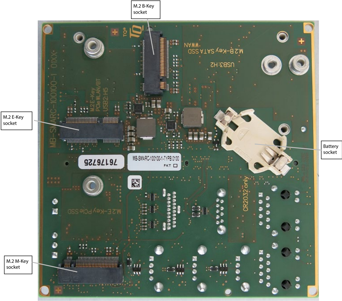
Figure 3: MB-SMARC-100100-1, Bottom
