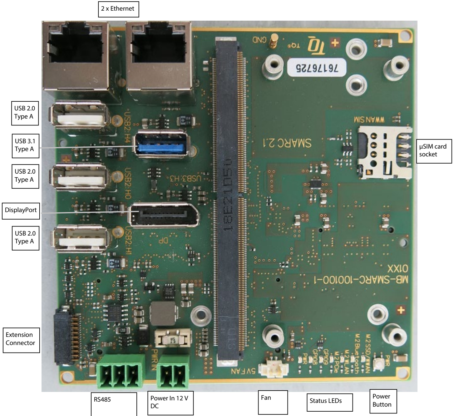
Figure 2: MB-SMARC-100100-1, Top
